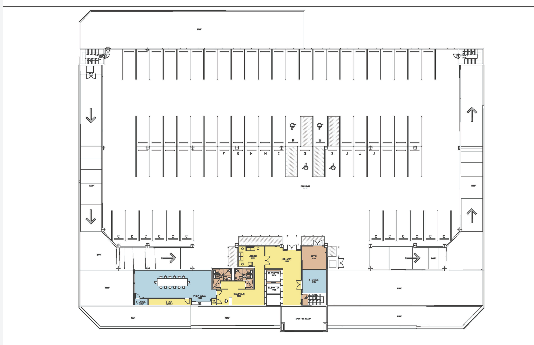
Proposed 2nd Floor Plan
