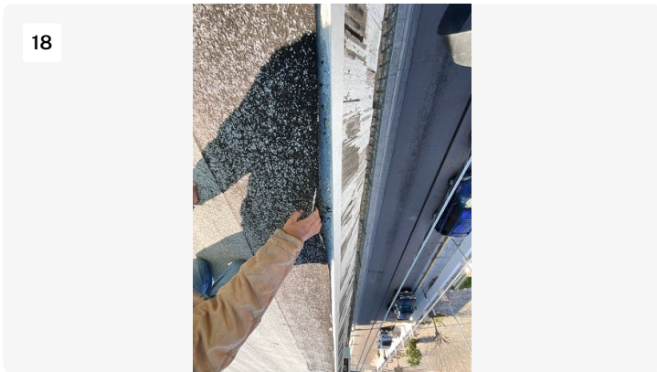
BUR membrane is detaching and coming undone
