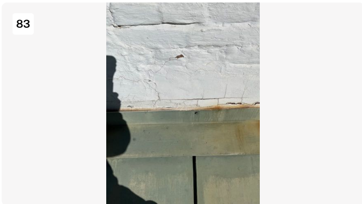
Fasteners coming undone and loose at counter flashing
