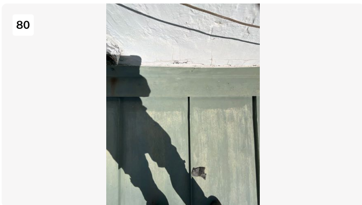
Voids on counter flashing sealant
