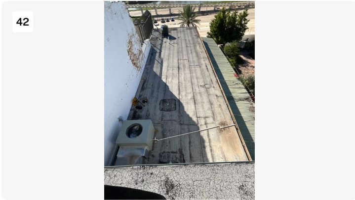
Discoloration and severe wear & tear on BUR membrane observed
