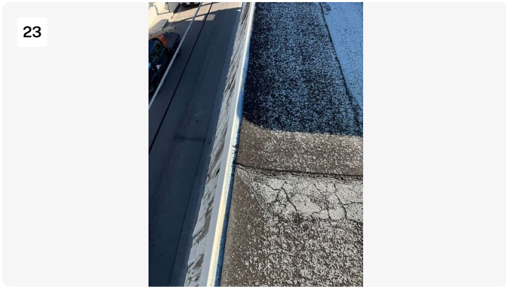
BUR membrane coming apart at roof edge/gutter transition
