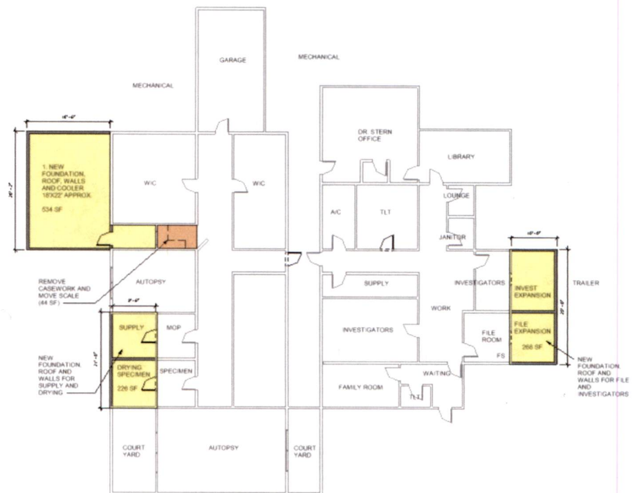
PRELIMINARY LAYOUT
