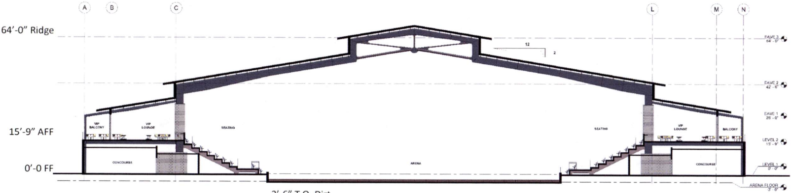
BUILDING SECTION
