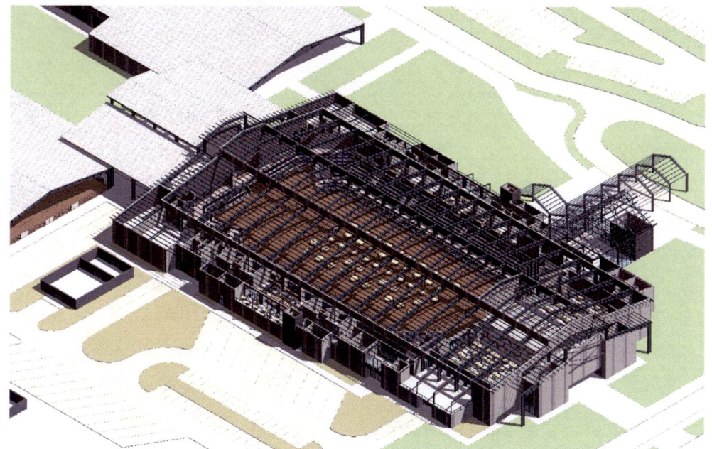
STRUCTURAL SYSTEM
