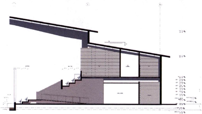
BUILDING SECTION @ VOMITORY
