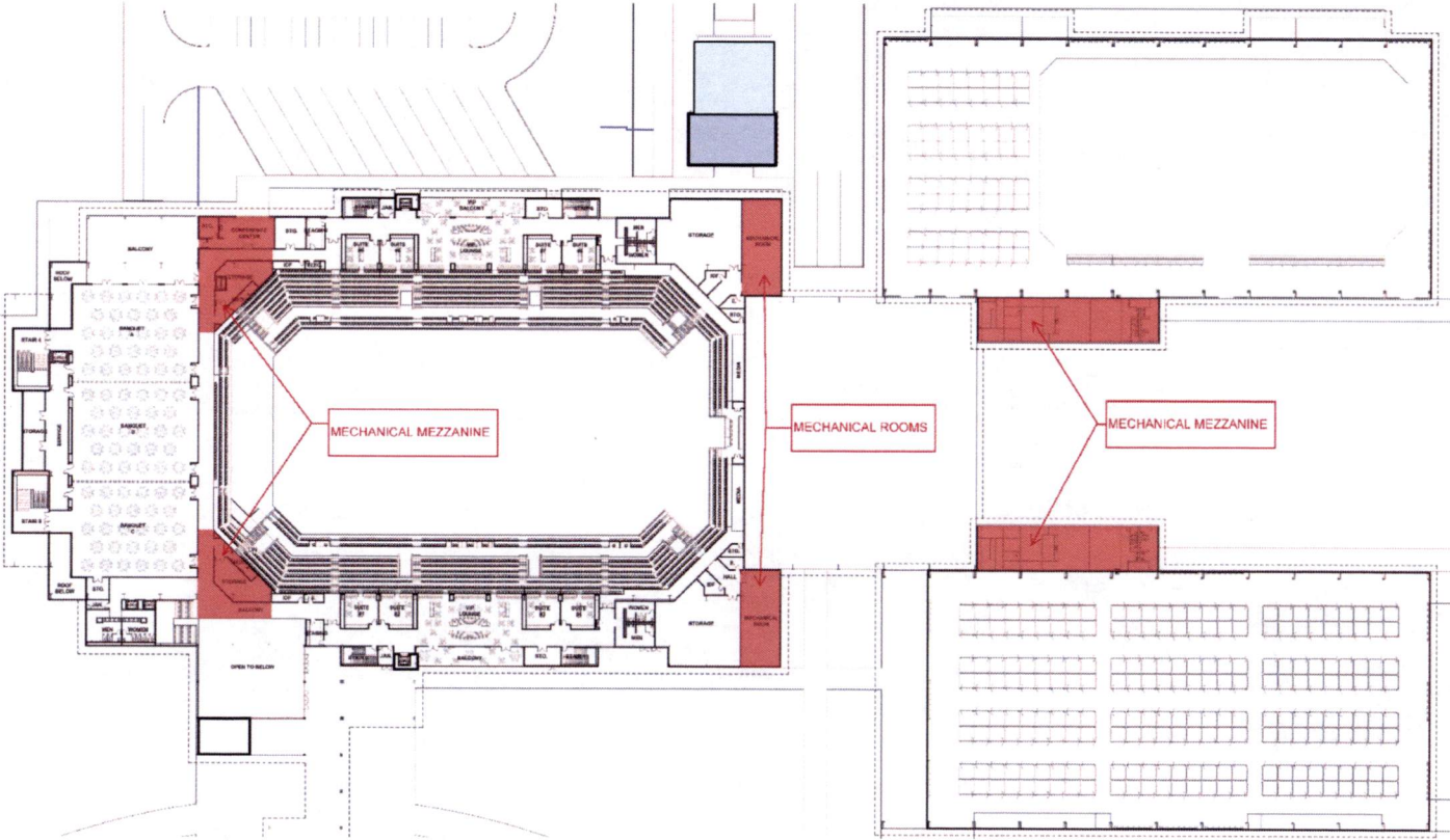
MEP SYSTEMS - CONCEPTUAL LAYOUTS
